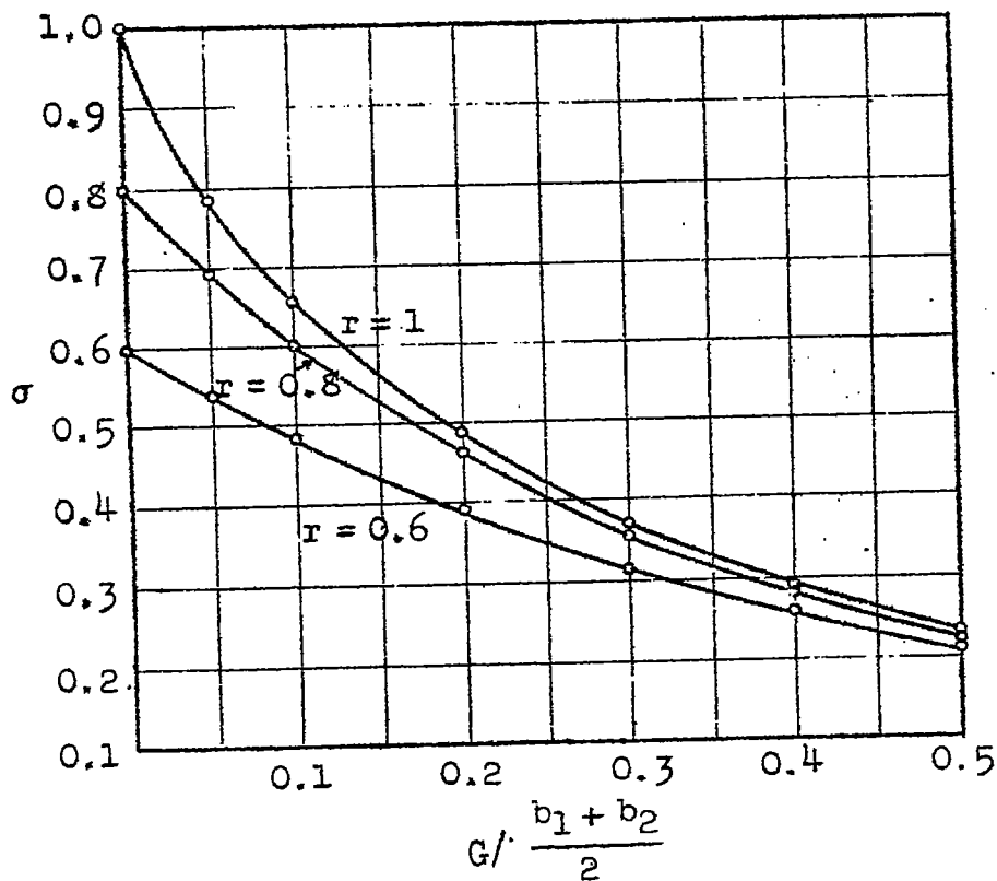
Fig.4. The coefficient of mutual influence \sigma plotted against G / \frac{b_1 + b_2}{2} . r = b_2 / b_1
