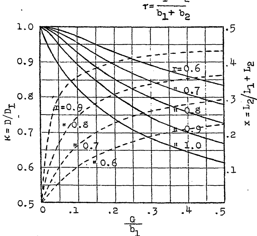
Fig.6. Distribution coefficient x and efficiency K of biplane plotted against G/b_1 , with r = b_2/b_1 .
